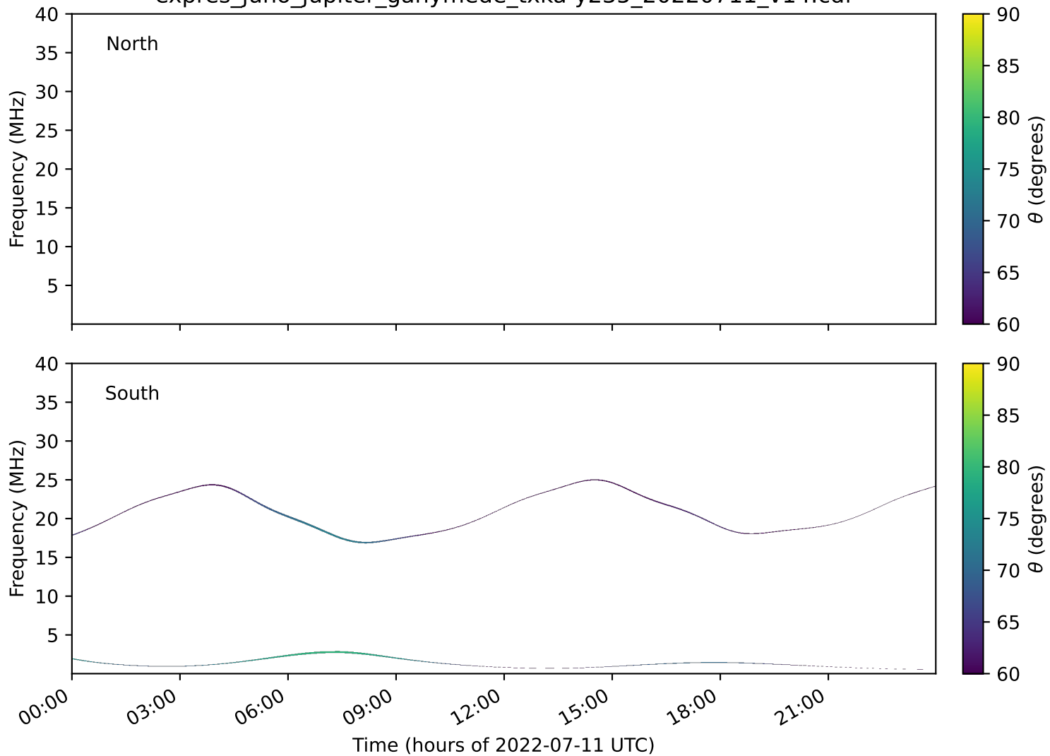
expres_juno_jupiter_ganymede_txka-y235_20220711_v14.cdf
