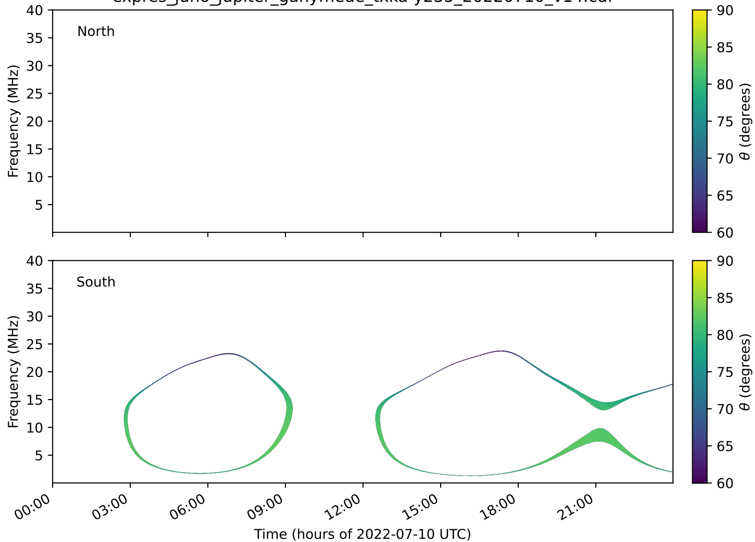
expres_juno_jupiter_ganymede_txka-y235_20220710_v14.cdf
