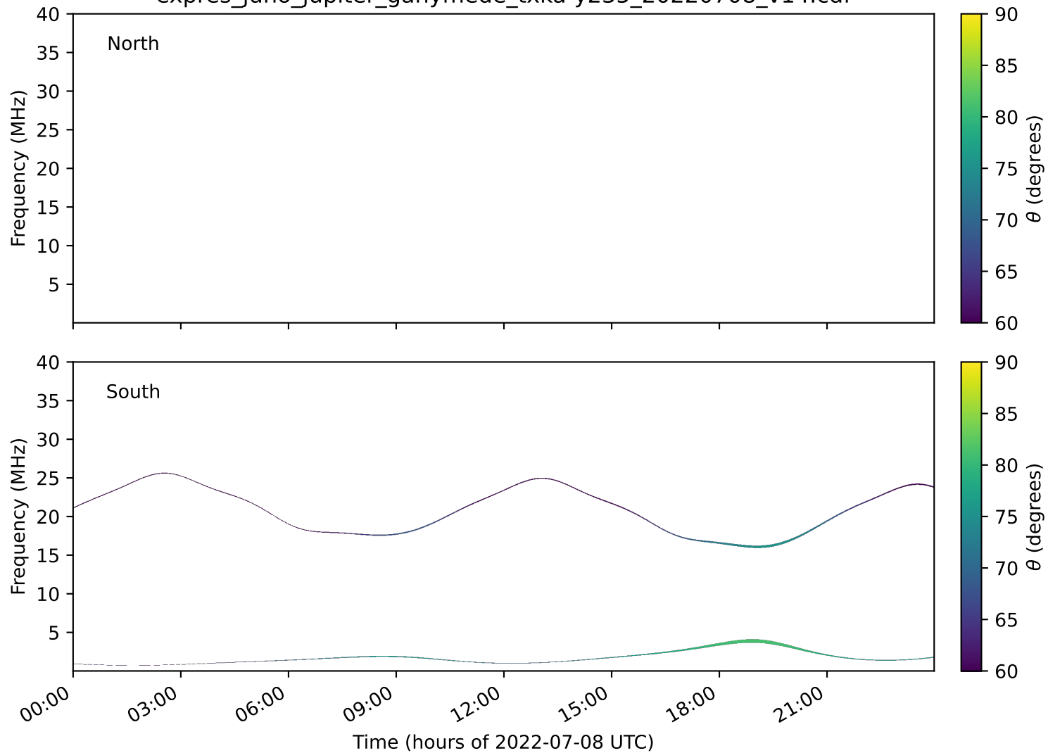
expres_juno_jupiter_ganymede_txka-y235_20220708_v14.cdf
