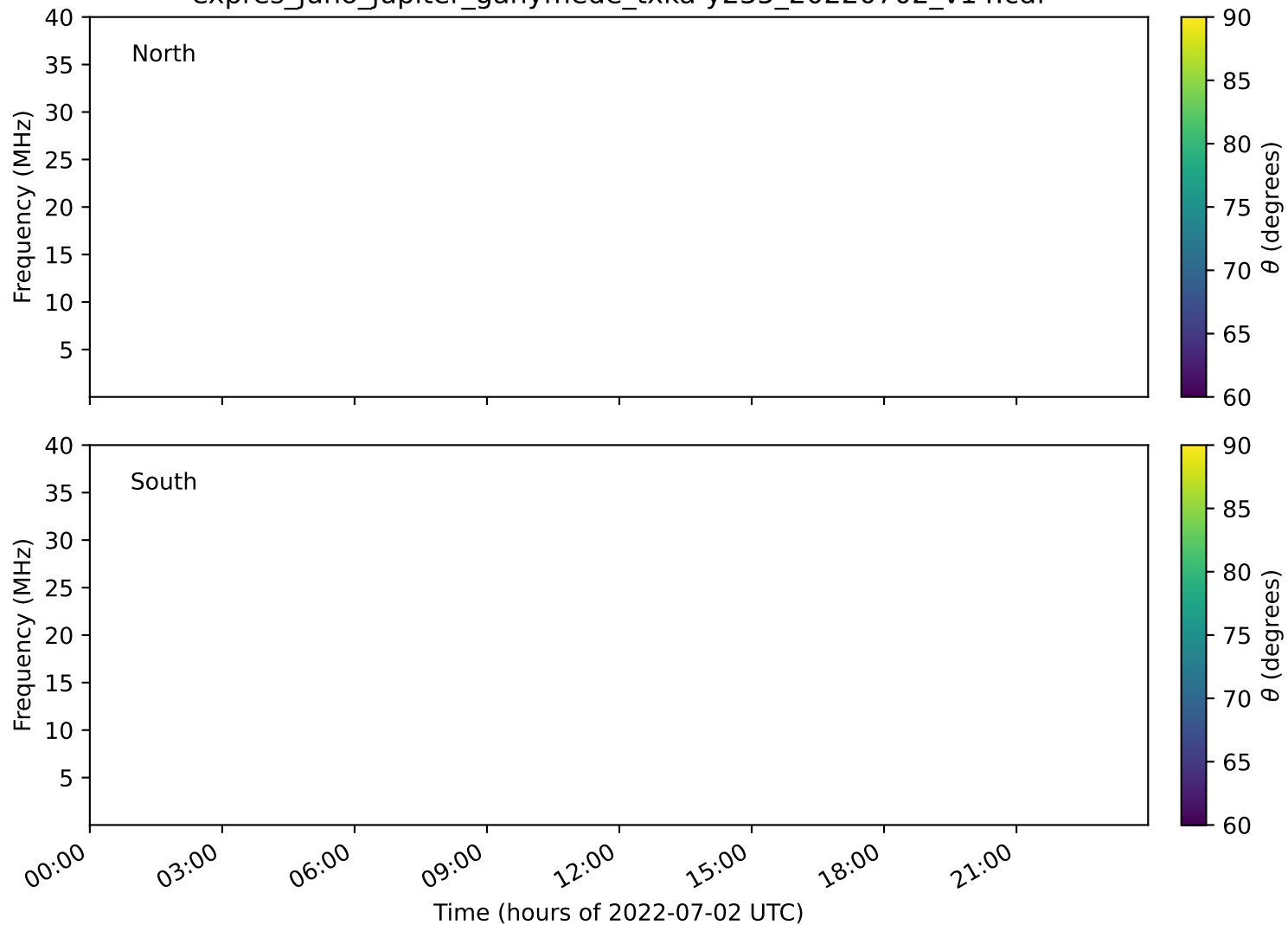
expres_juno_jupiter_ganymede_txka-y235_20220702_v14.cdf
