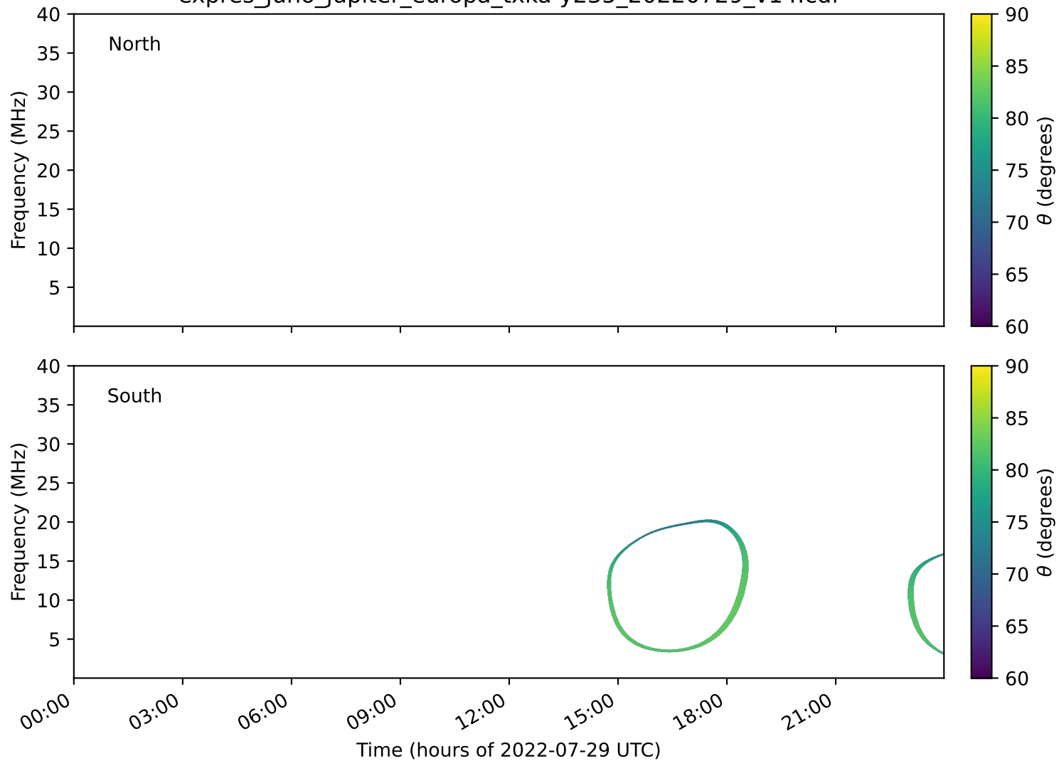
expres_juno_jupiter_europa_txka-y235_20220729_v14.cdf
