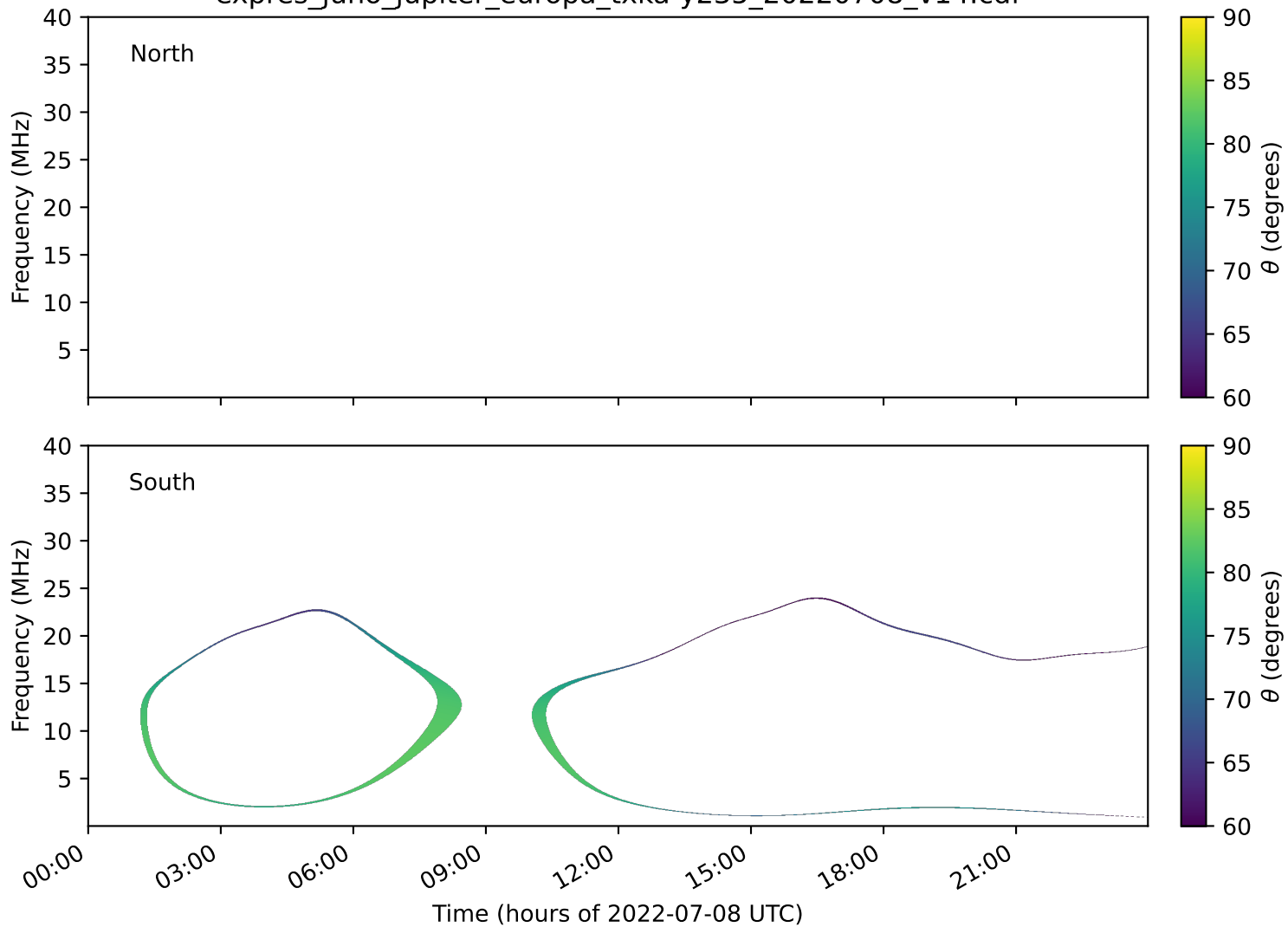
expres_juno_jupiter_europa_txka-y235_20220708_v14.cdf
