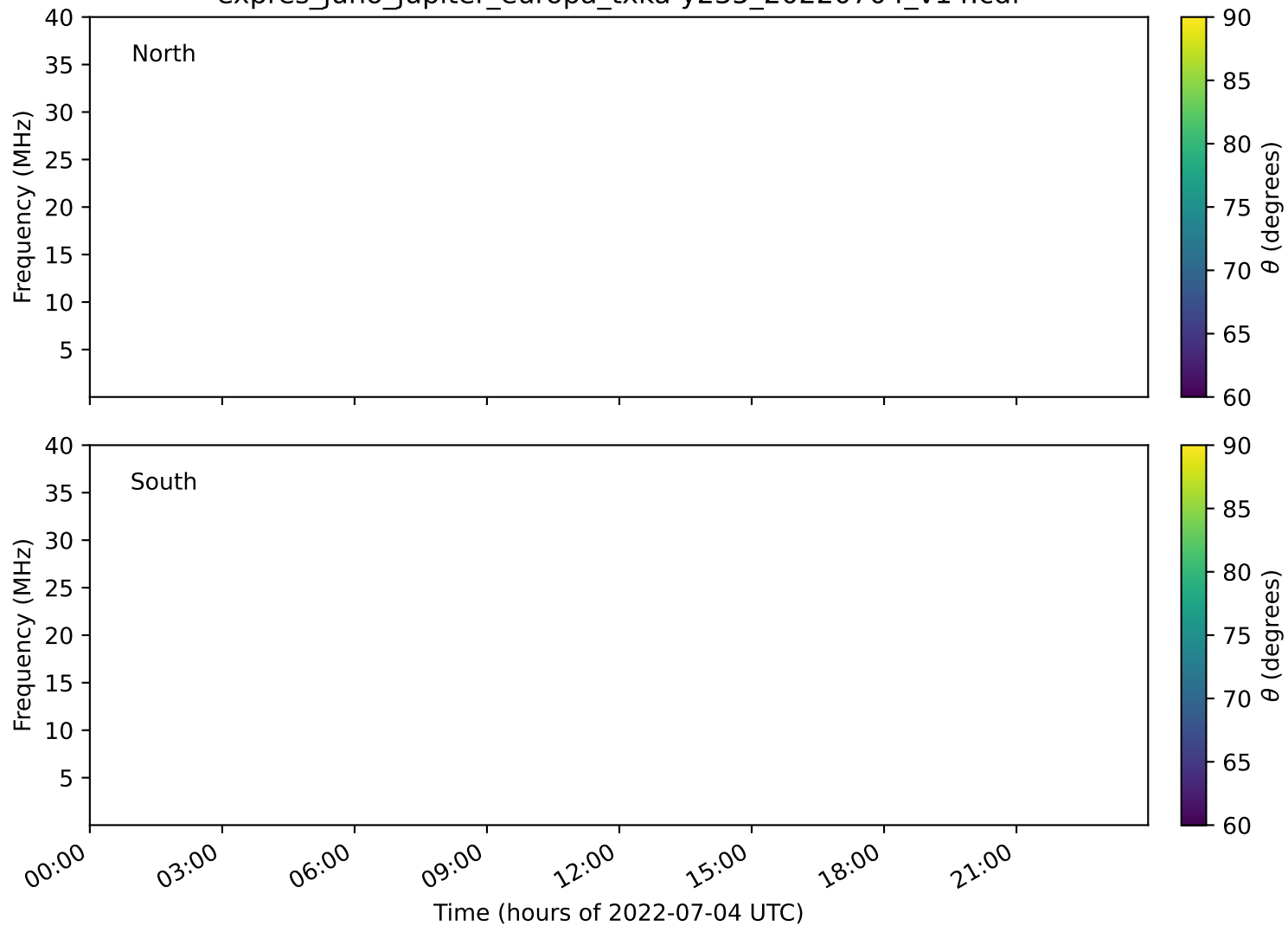
expres_juno_jupiter_europa_txka-y235_20220704_v14.cdf
