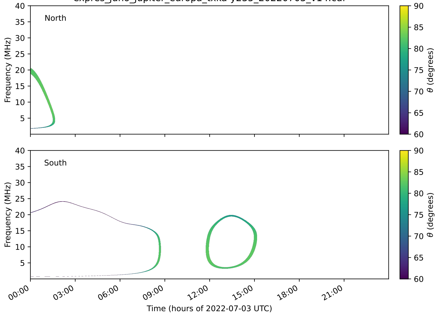
expres_juno_jupiter_europa_txka-y235_20220703_v14.cdf
