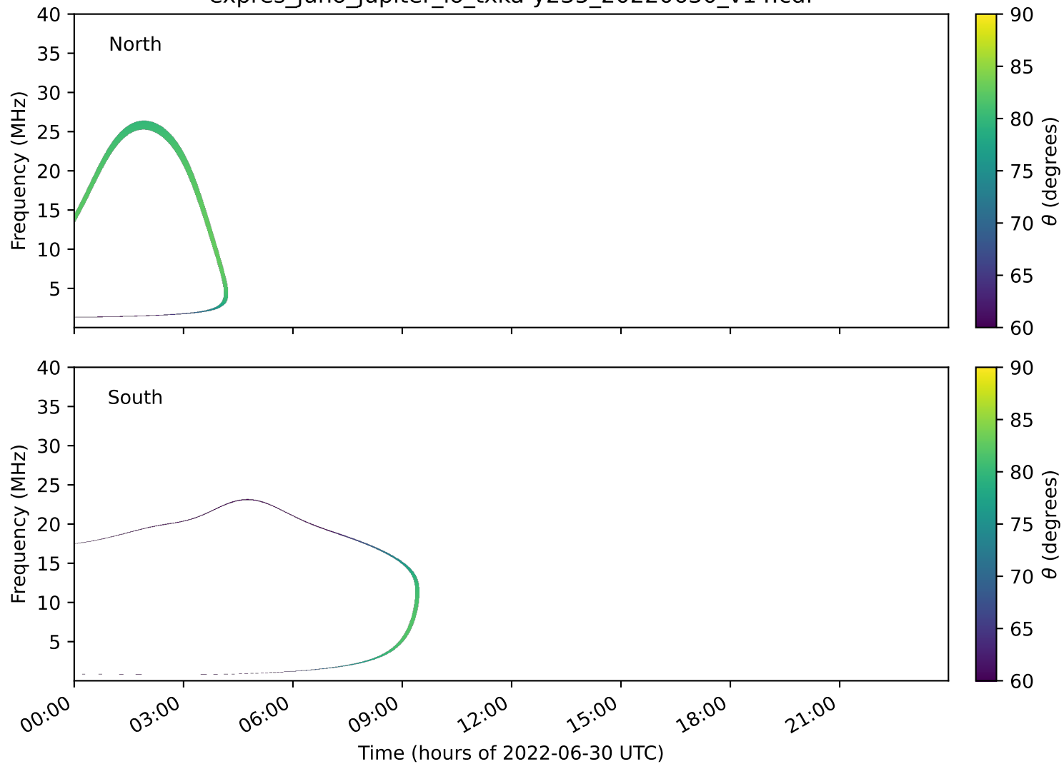
expres_juno_jupiter_io_txka-y235_20220630_v14.cdf
