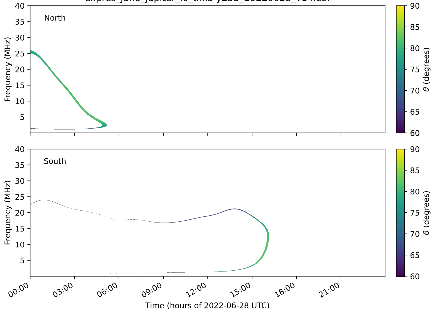
expres_juno_jupiter_io_txka-y235_20220628_v14.cdf
