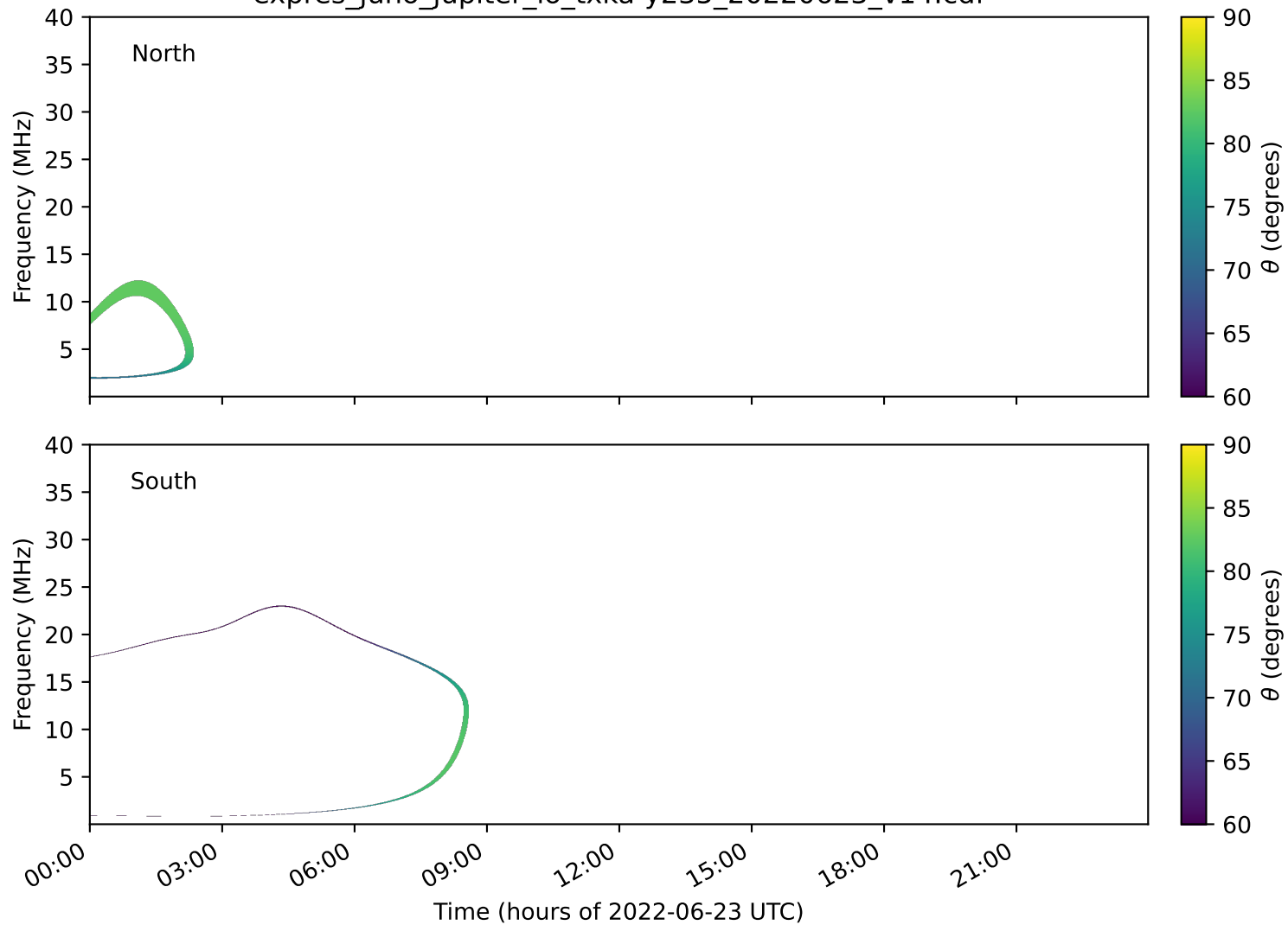
expres_juno_jupiter_io_txka-y235_20220623_v14.cdf
