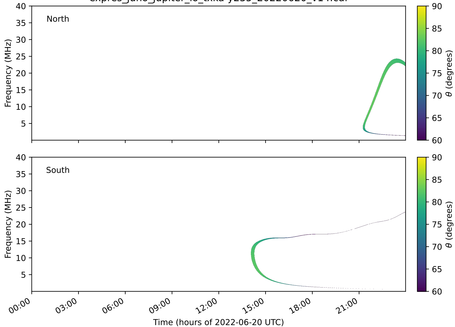
expres_juno_jupiter_io_txka-y235_20220620_v14.cdf
