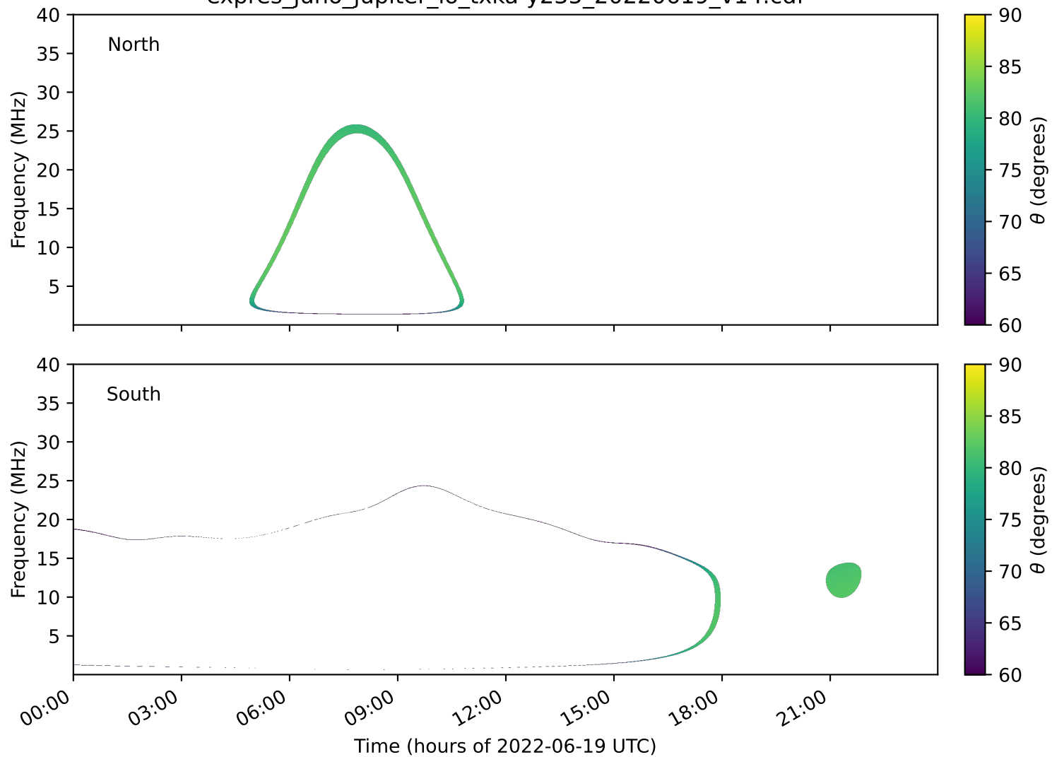
expres_juno_jupiter_io_txka-y235_20220619_v14.cdf
