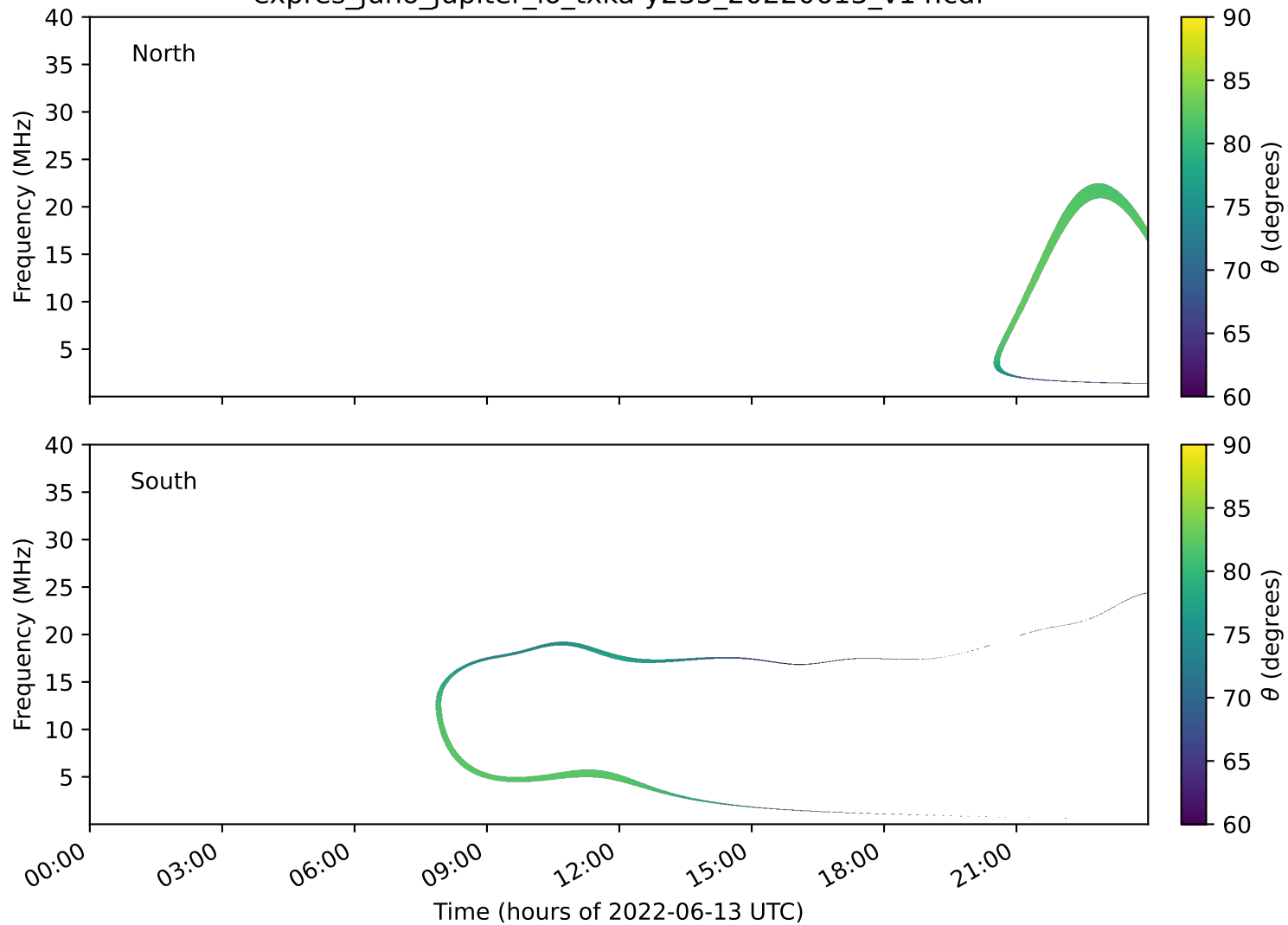
expres_juno_jupiter_io_txka-y235_20220613_v14.cdf
