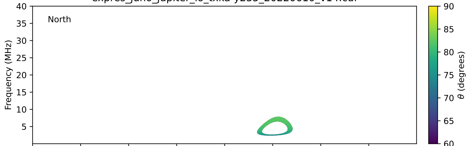
expres_juno_jupiter_io_txka-y235_20220610_v14.cdf
