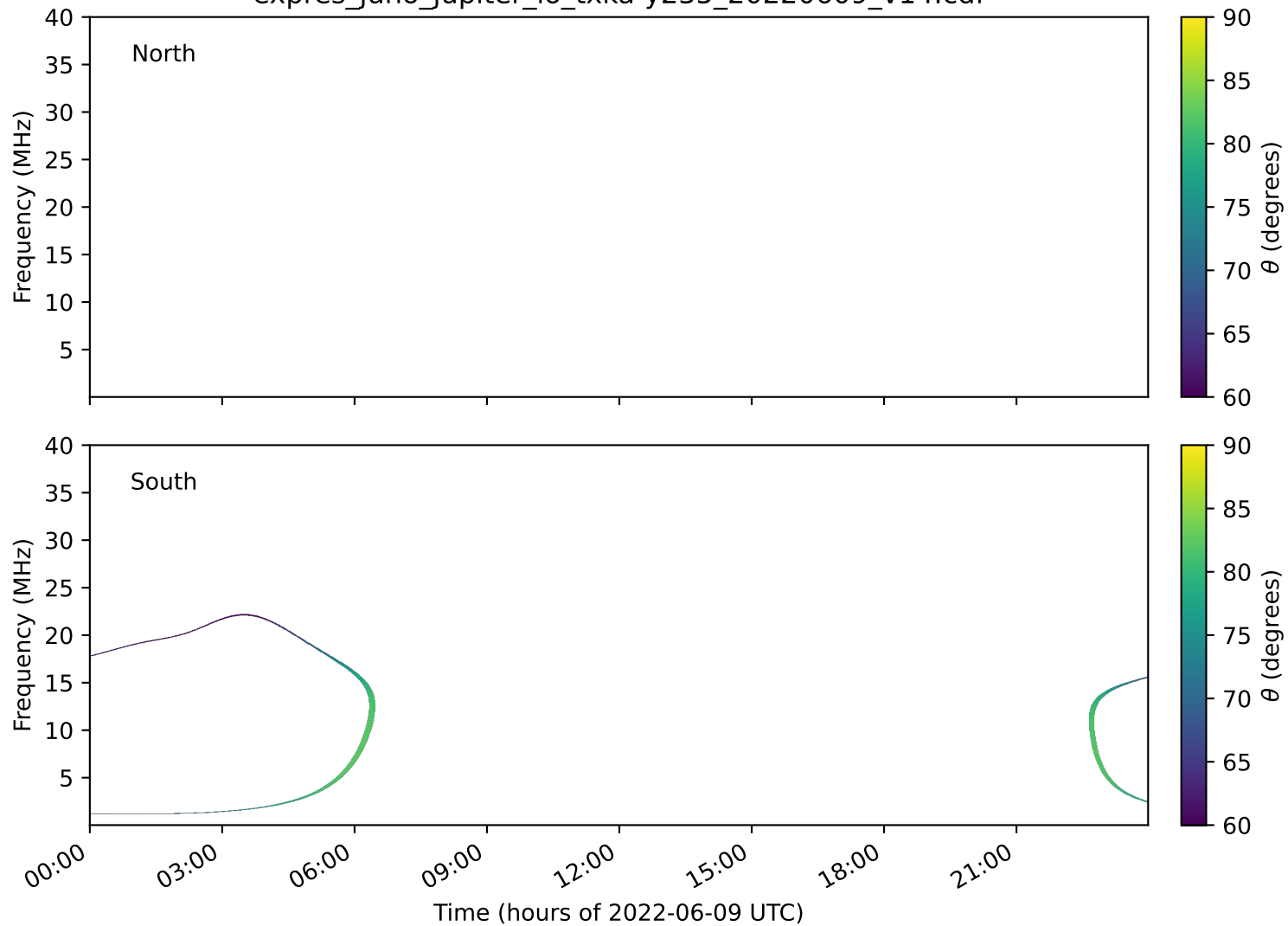
expres_juno_jupiter_io_txka-y235_20220609_v14.cdf
