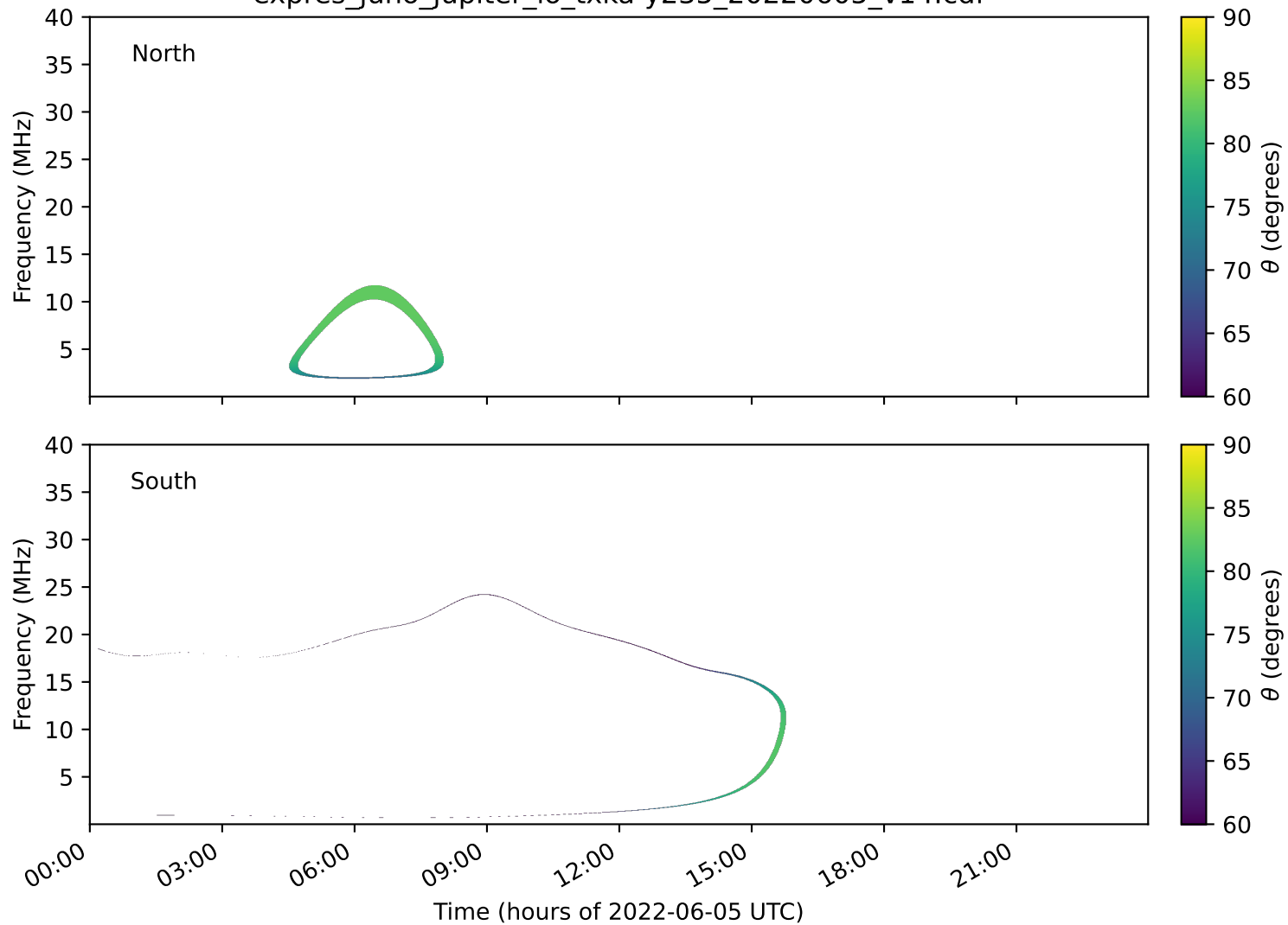
expres_juno_jupiter_io_txka-y235_20220605_v14.cdf
