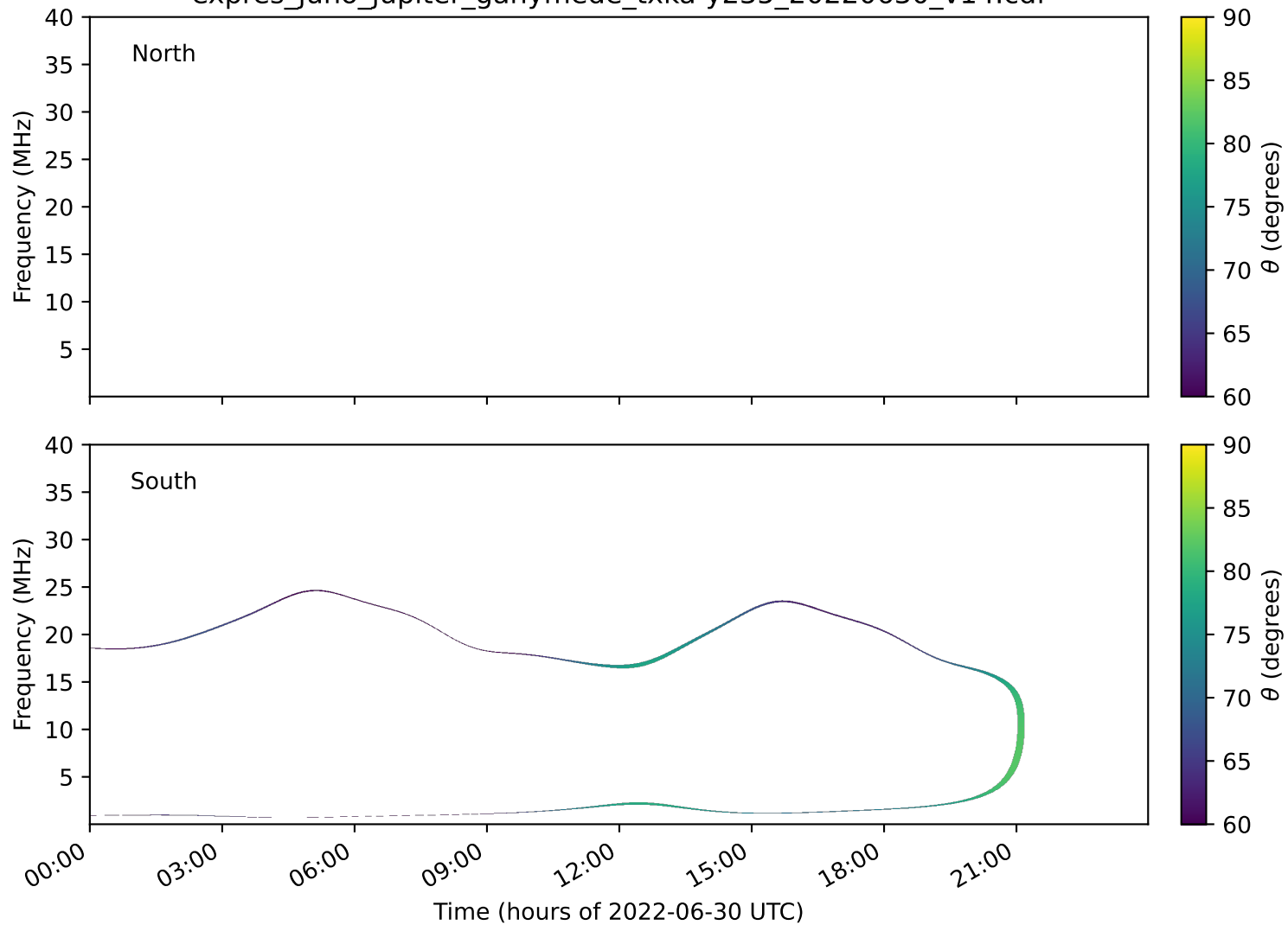
expres_juno_jupiter_ganymede_txka-y235_20220630_v14.cdf
