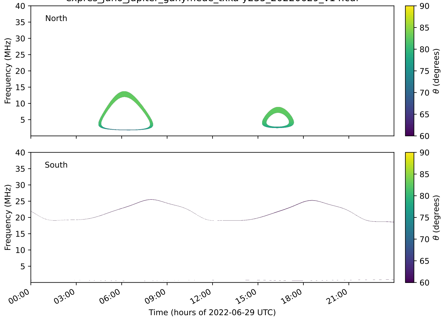
expres_juno_jupiter_ganymede_txka-y235_20220629_v14.cdf
