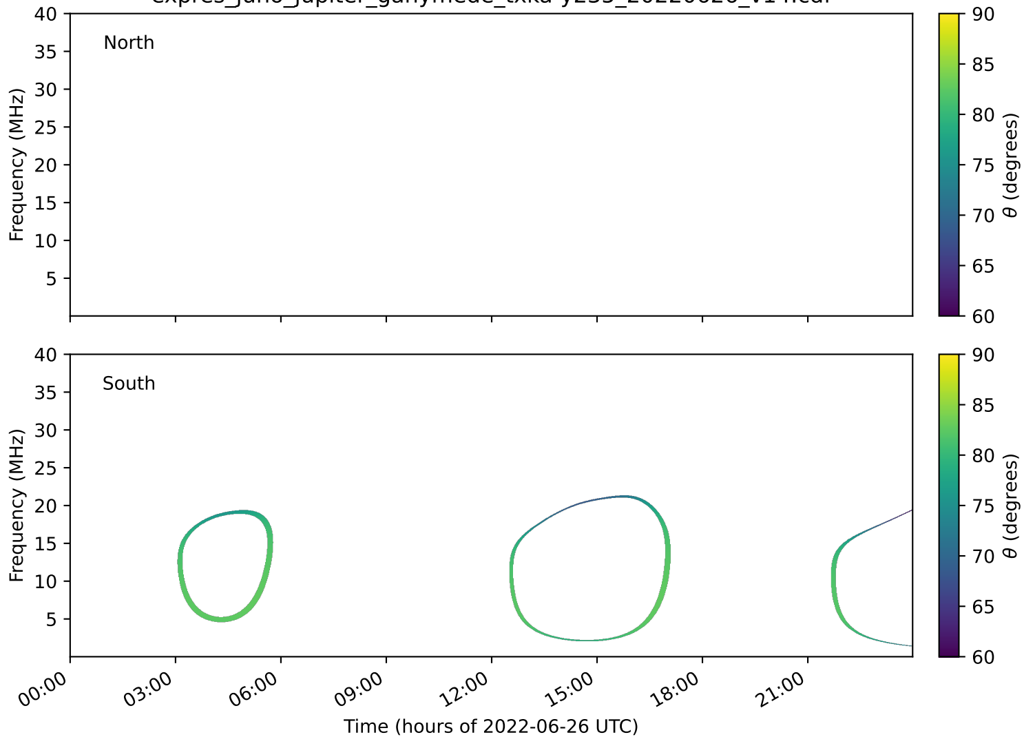
expres_juno_jupiter_ganymede_txka-y235_20220626_v14.cdf
