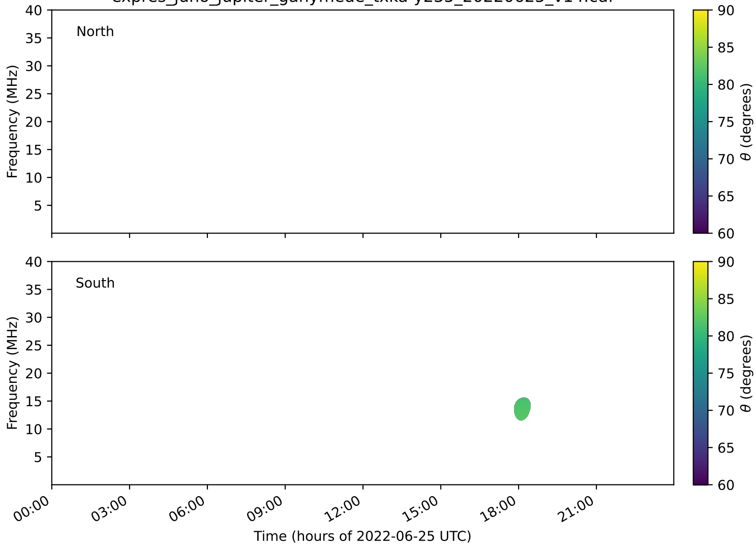
expres_juno_jupiter_ganymede_txka-y235_20220625_v14.cdf
