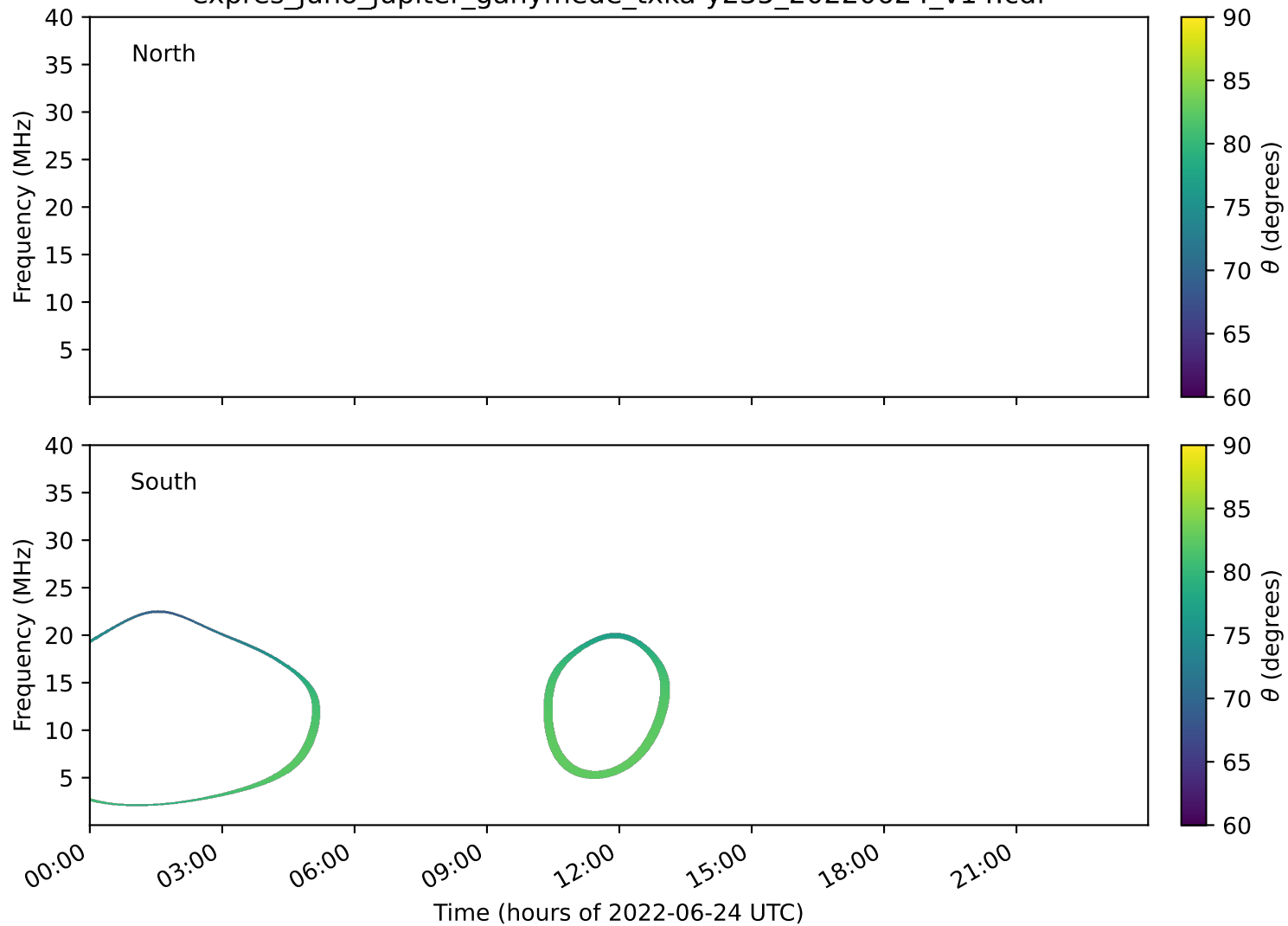
expres_juno_jupiter_ganymede_txka-y235_20220624_v14.cdf
