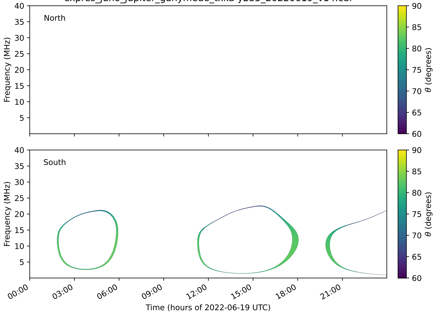
expres_juno_jupiter_ganymede_txka-y235_20220619_v14.cdf
