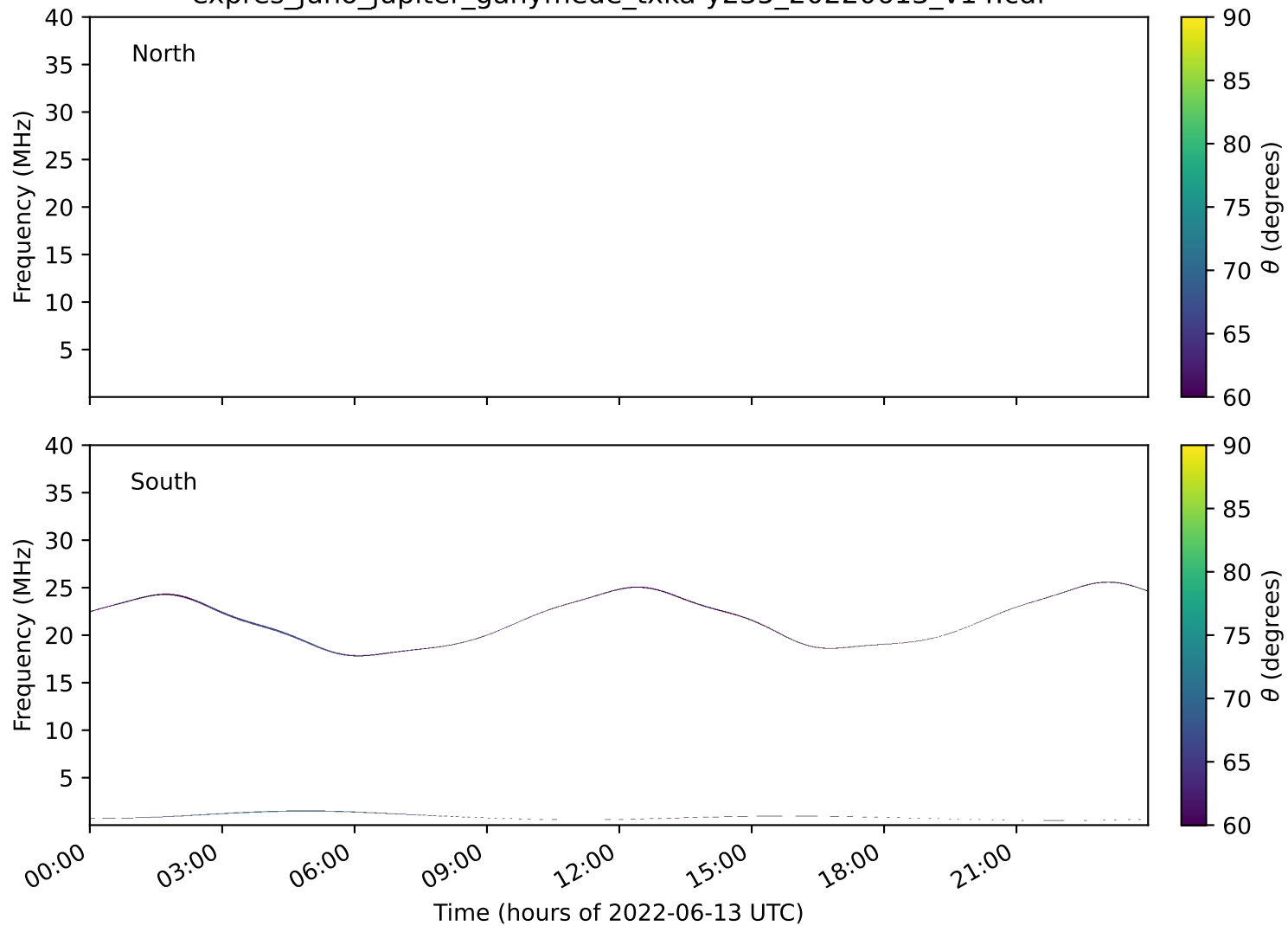
expres_juno_jupiter_ganymede_txka-y235_20220613_v14.cdf
