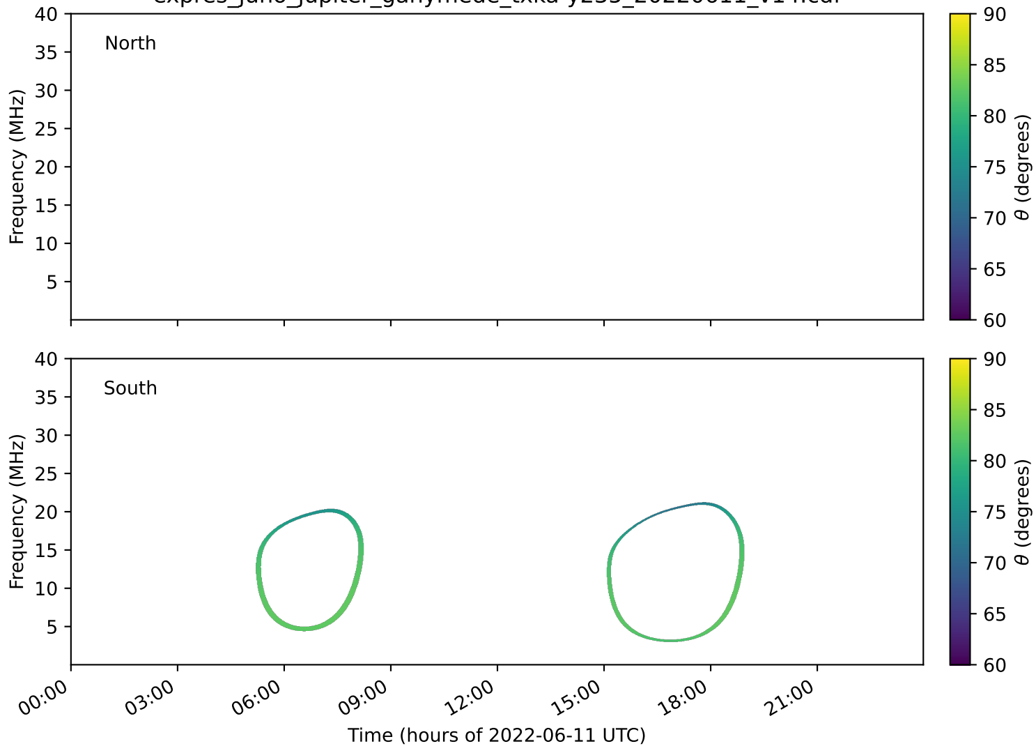
expres_juno_jupiter_ganymede_txka-y235_20220611_v14.cdf
