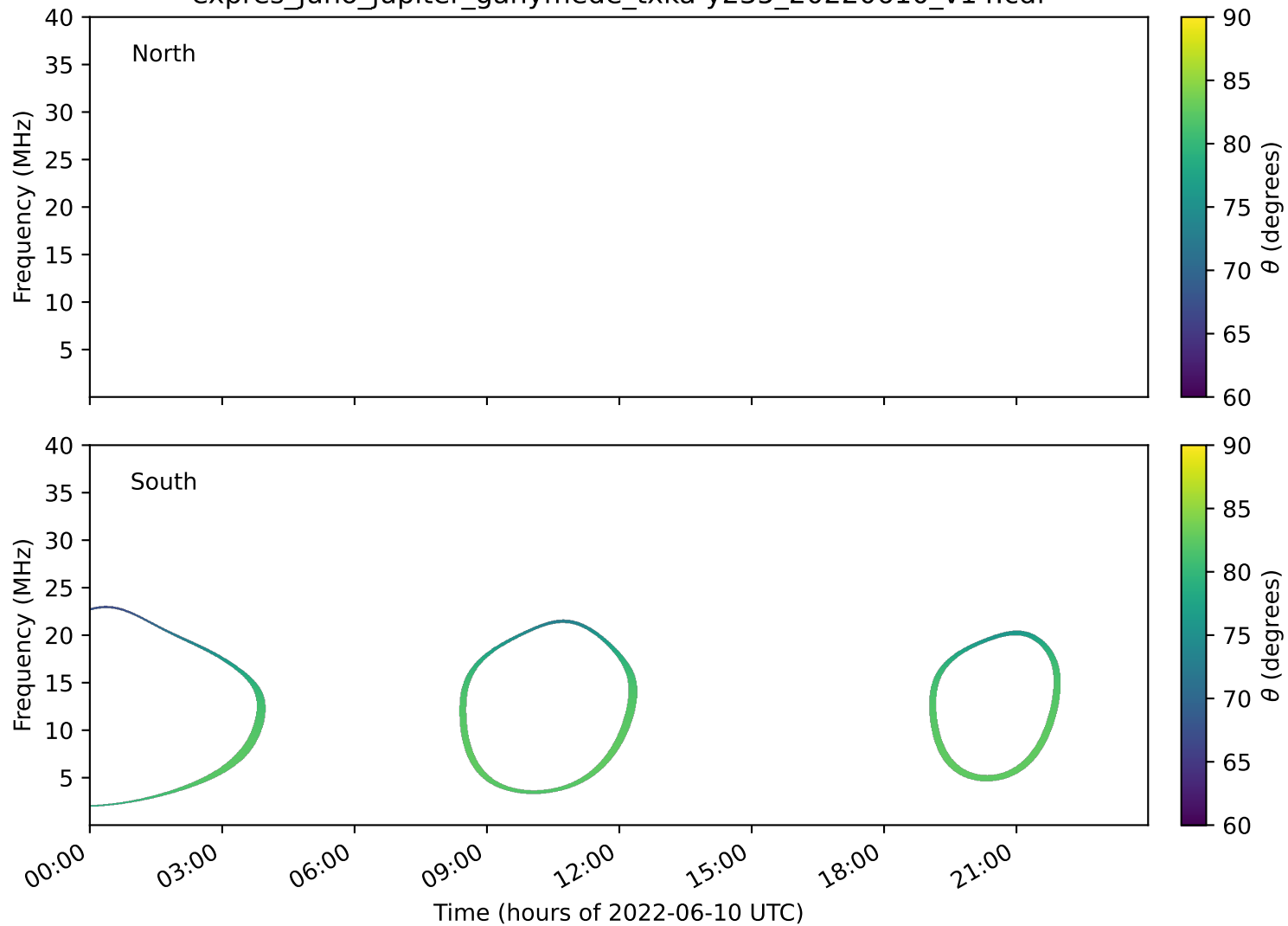
expres_juno_jupiter_ganymede_txka-y235_20220610_v14.cdf
