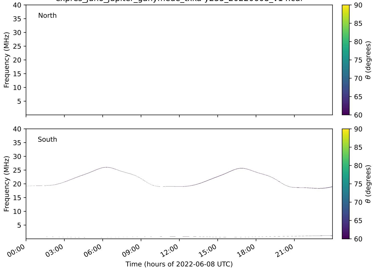
expres_juno_jupiter_ganymede_txka-y235_20220608_v14.cdf
