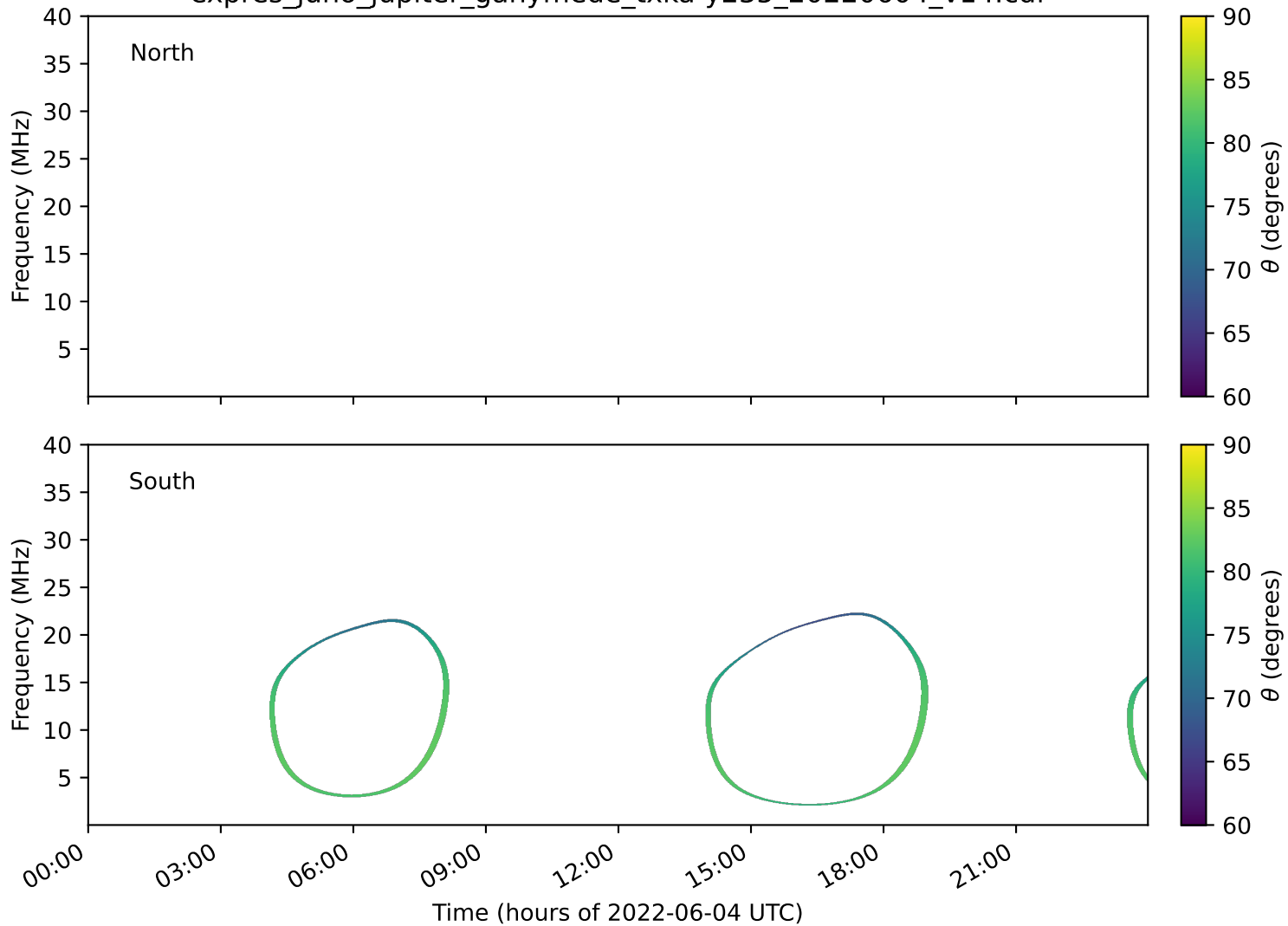
expres_juno_jupiter_ganymede_txka-y235_20220604_v14.cdf
