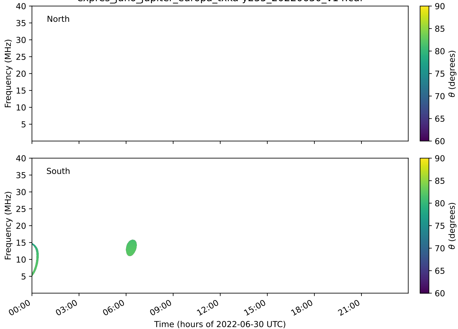
expres_juno_jupiter_europa_txka-y235_20220630_v14.cdf
