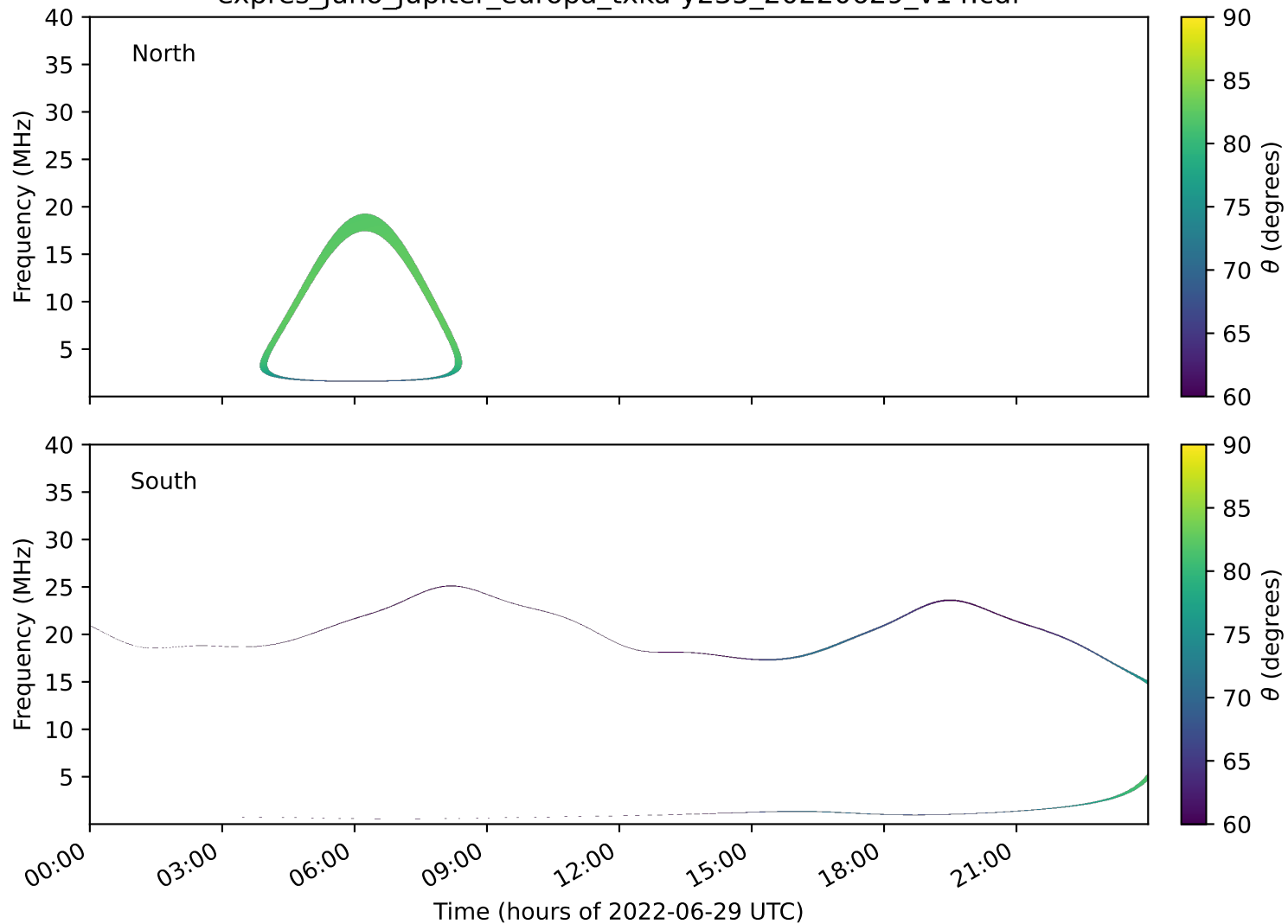
expres_juno_jupiter_europa_txka-y235_20220629_v14.cdf
