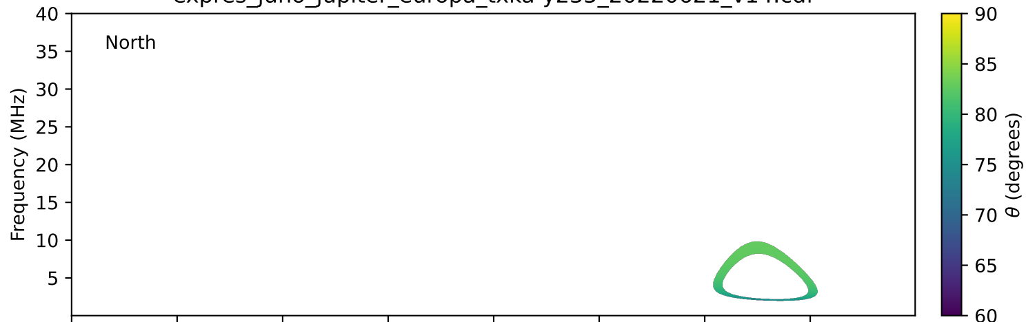
expres_juno_jupiter_europa_txka-y235_20220621_v14.cdf
