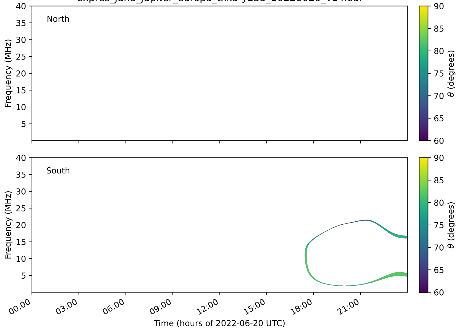
expres_juno_jupiter_europa_txka-y235_20220620_v14.cdf
