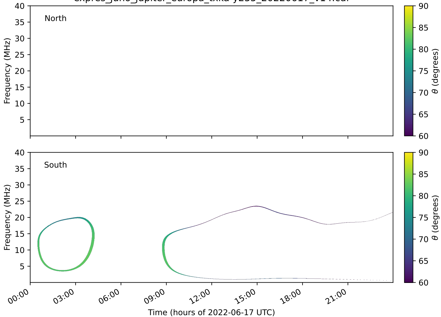
expres_juno_jupiter_europa_txka-y235_20220617_v14.cdf
