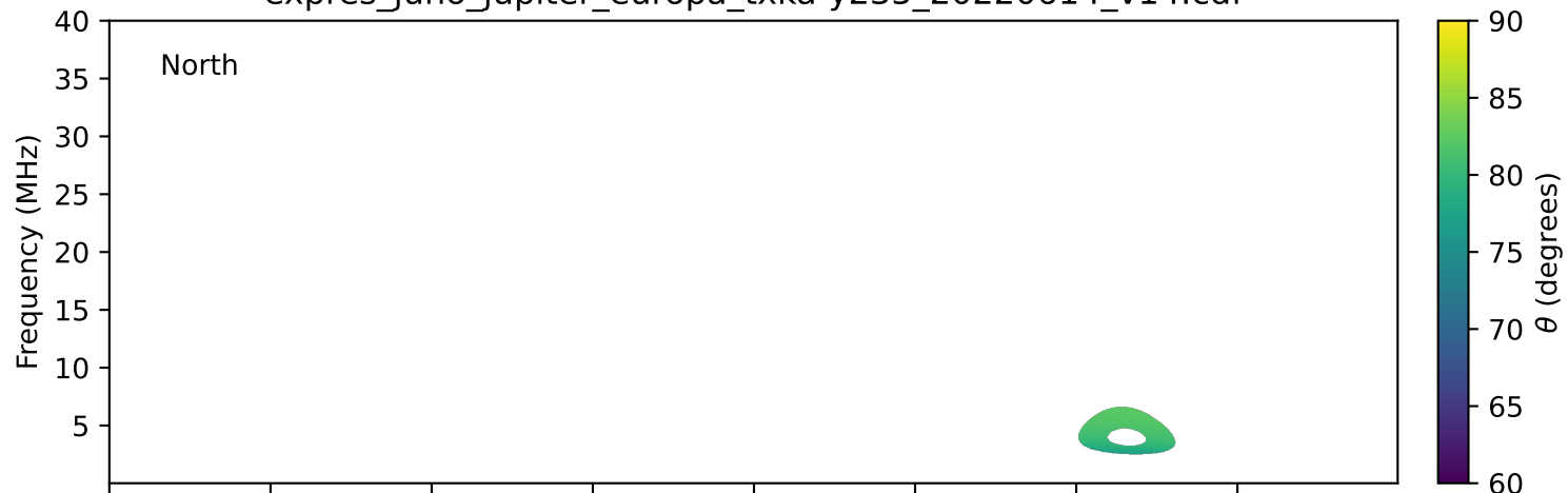
expres_juno_jupiter_europa_txka-y235_20220614_v14.cdf
