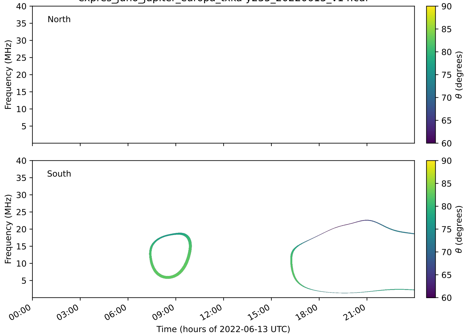
expres_juno_jupiter_europa_txka-y235_20220613_v14.cdf
