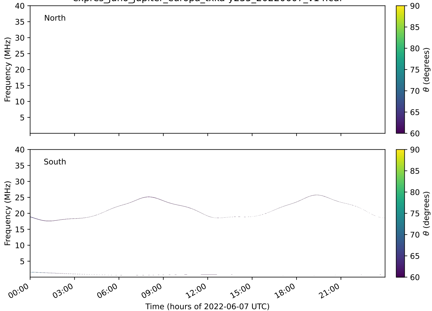
expres_juno_jupiter_europa_txka-y235_20220607_v14.cdf
