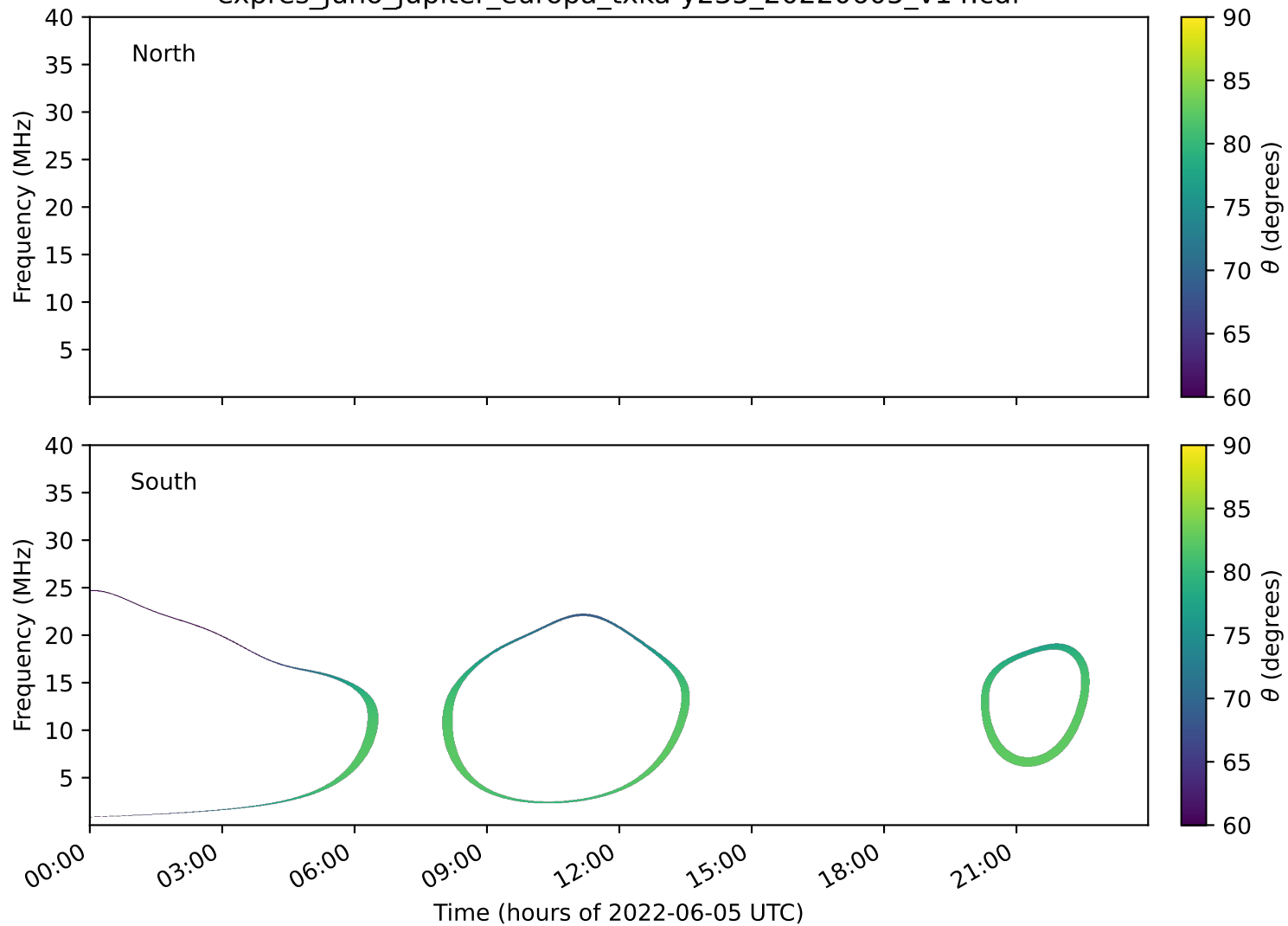
expres_juno_jupiter_europa_txka-y235_20220605_v14.cdf
