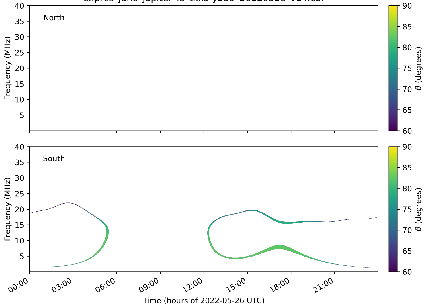
expres_juno_jupiter_io_txka-y235_20220526_v14.cdf
