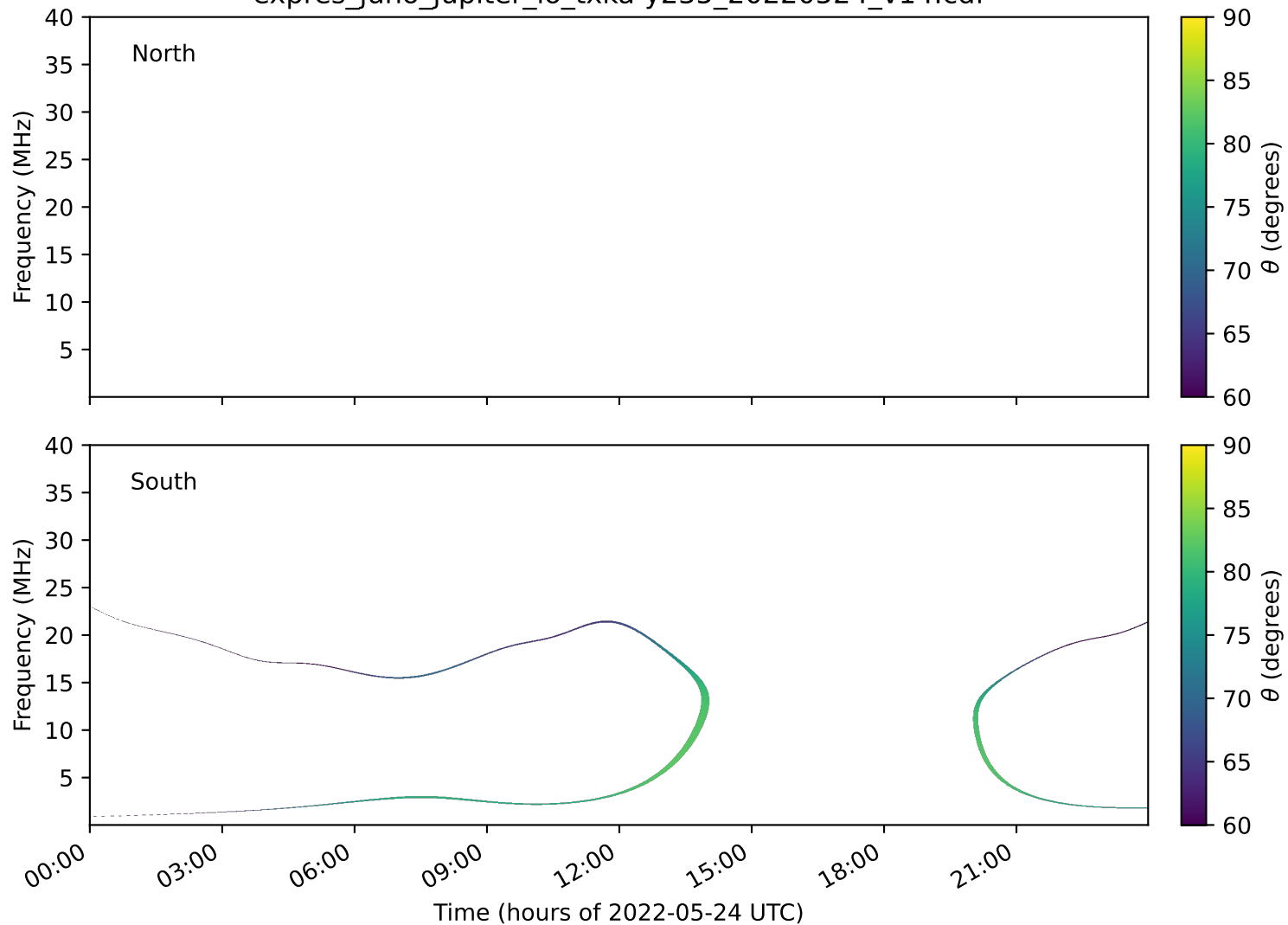
expres_juno_jupiter_io_txka-y235_20220524_v14.cdf
