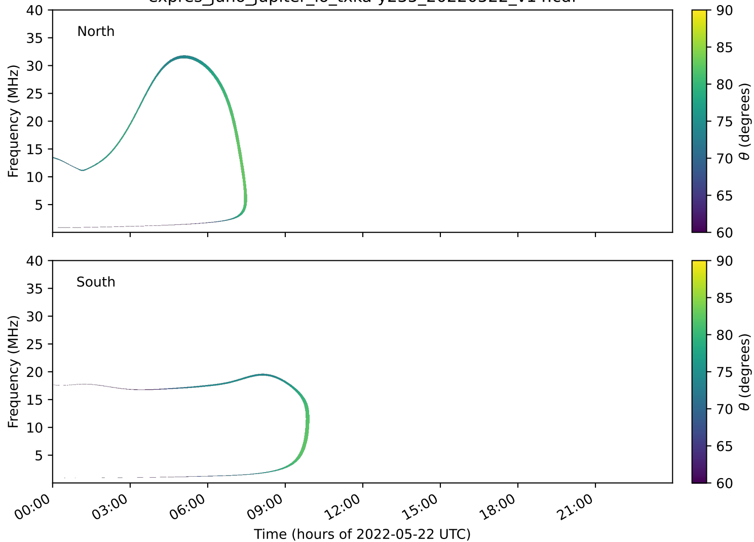
expres_juno_jupiter_io_txka-y235_20220522_v14.cdf
