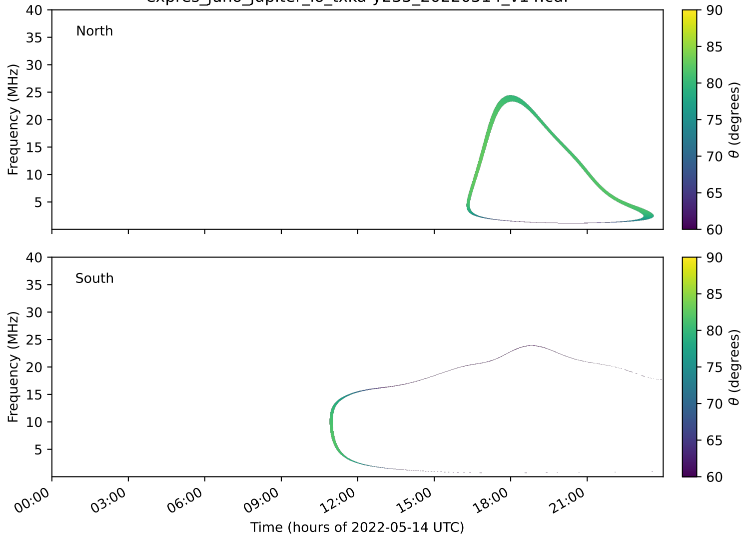
expres_juno_jupiter_io_txka-y235_20220514_v14.cdf
