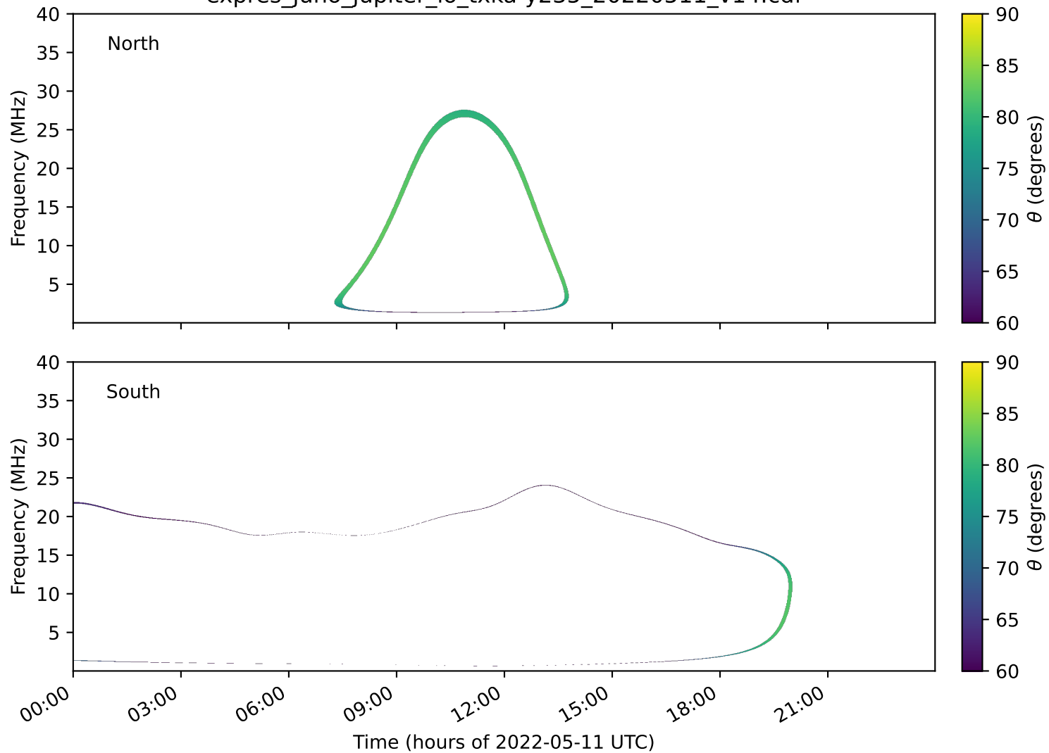
expres_juno_jupiter_io_txka-y235_20220511_v14.cdf
