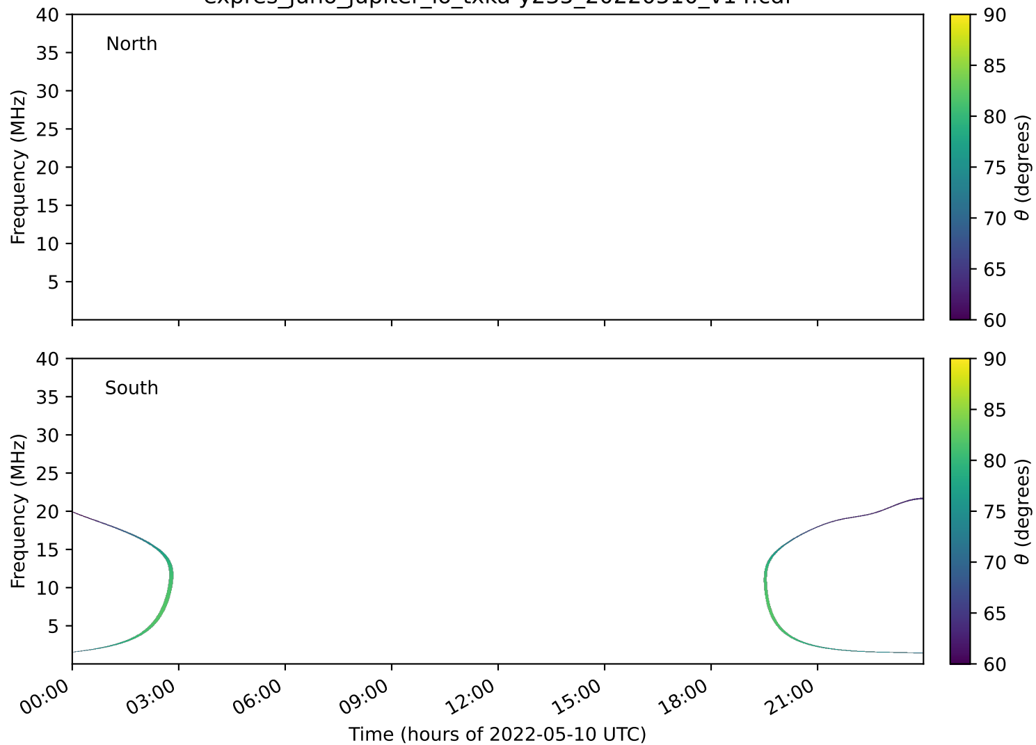
expres_juno_jupiter_io_txka-y235_20220510_v14.cdf
