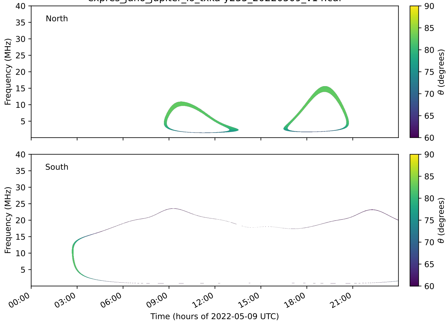
expres_juno_jupiter_io_txka-y235_20220509_v14.cdf
