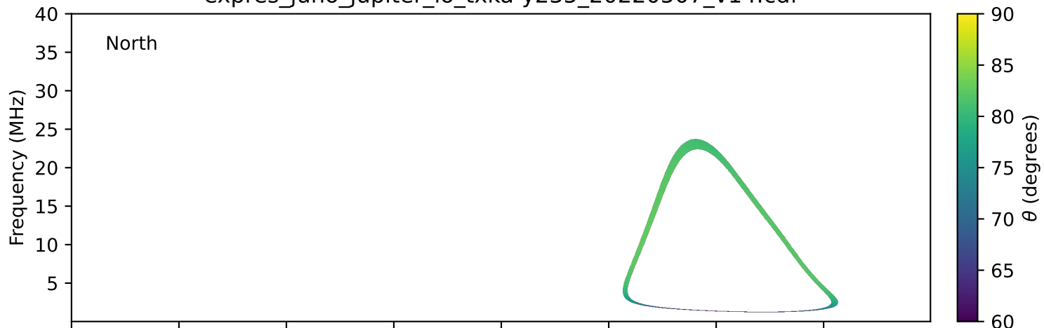
expres_juno_jupiter_io_txka-y235_20220507_v14.cdf
