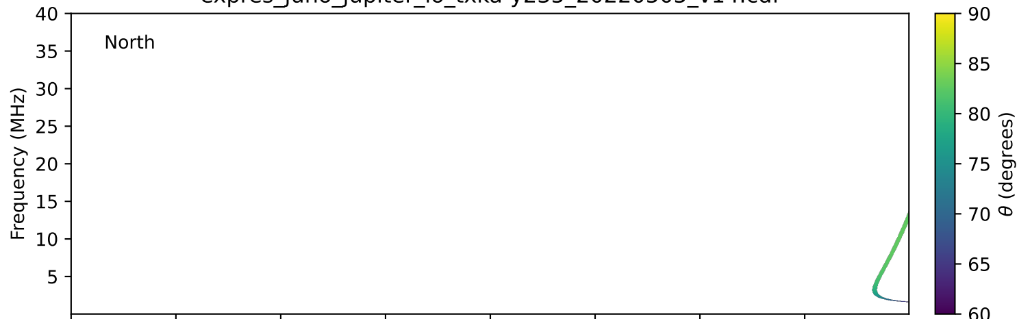
expres_juno_jupiter_io_txka-y235_20220505_v14.cdf
