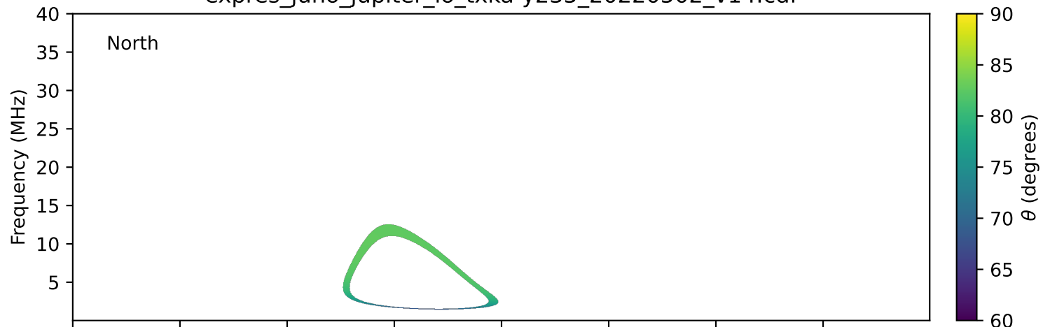
expres_juno_jupiter_io_txka-y235_20220502_v14.cdf
