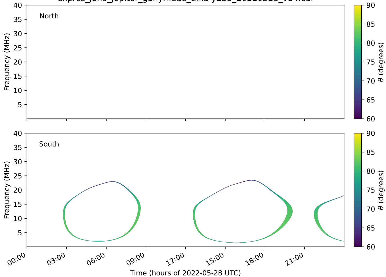
expres_juno_jupiter_ganymede_txka-y235_20220528_v14.cdf
