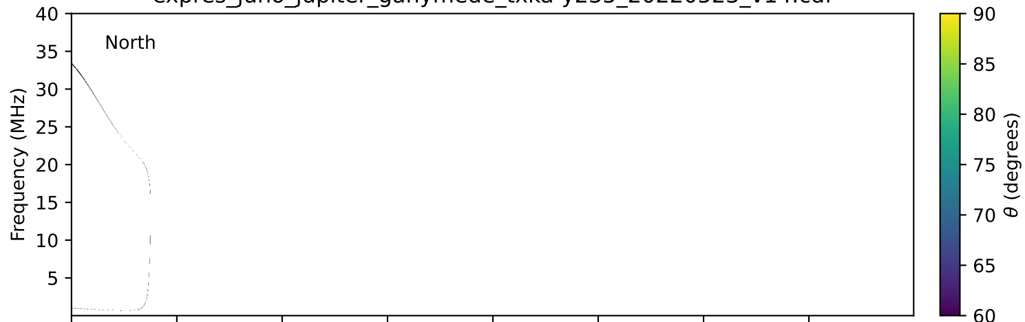
expres_juno_jupiter_ganymede_txka-y235_20220523_v14.cdf
