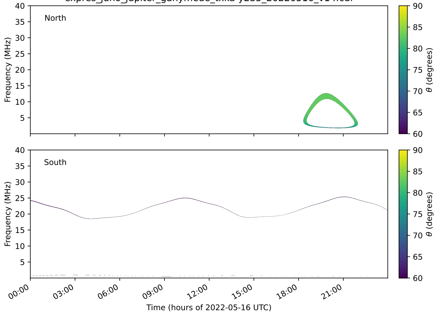
expres_juno_jupiter_ganymede_txka-y235_20220516_v14.cdf
